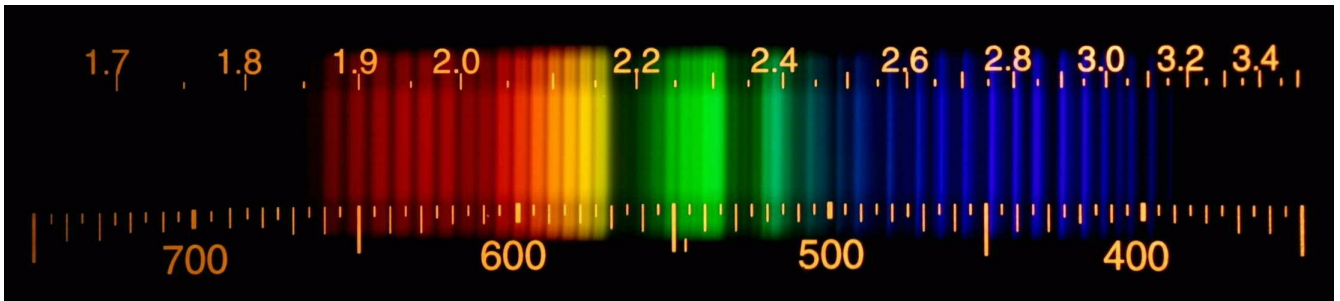
Nitrogen (N)
