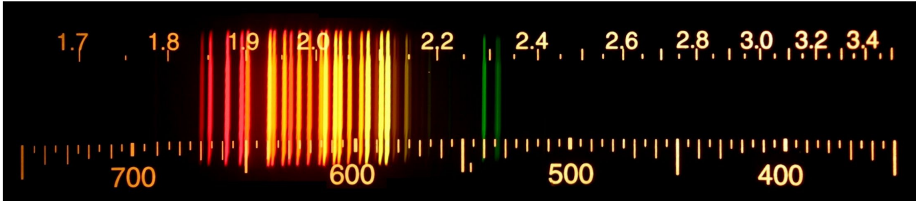
Neon (Ne)
