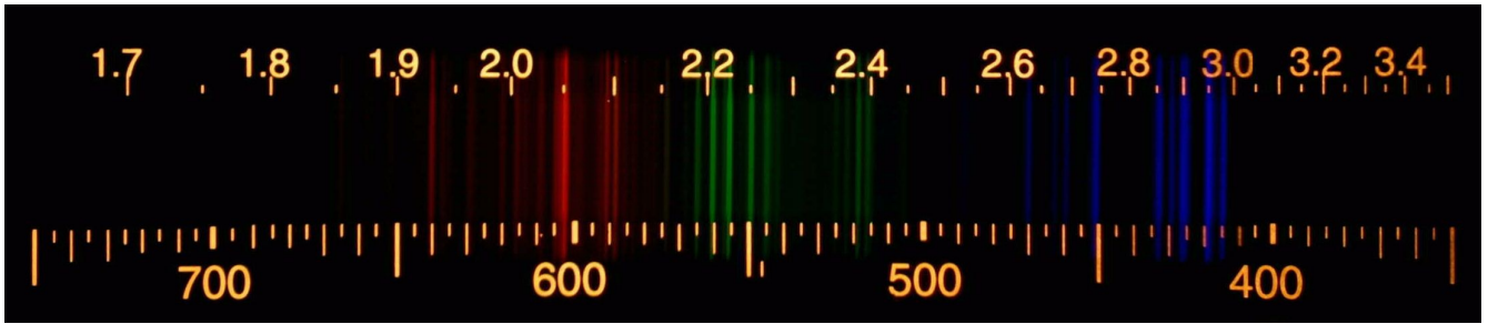
Argon (Ar)
